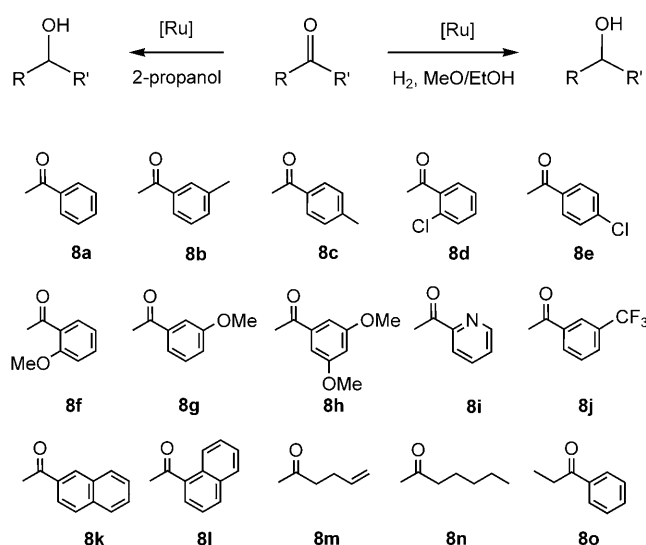
Scheme 3. Asymmetric TH and HY of ketones catalyzed by the chiral pincer complexes 2–7 .
