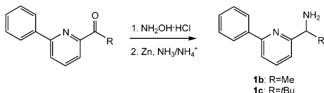
Scheme 1. Synthesis of the ligands 1b and 1c .
