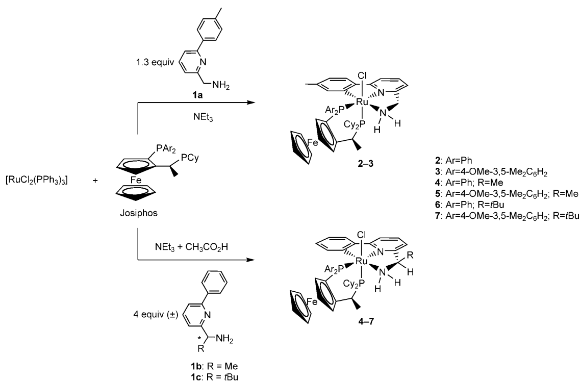
Scheme 2. Synthesis of the chiral pincer CNN complexes 2–7 .
